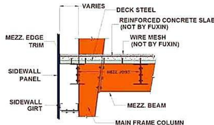
MEZZ. BEAM CONNECTION TO MAIN COLUMN
