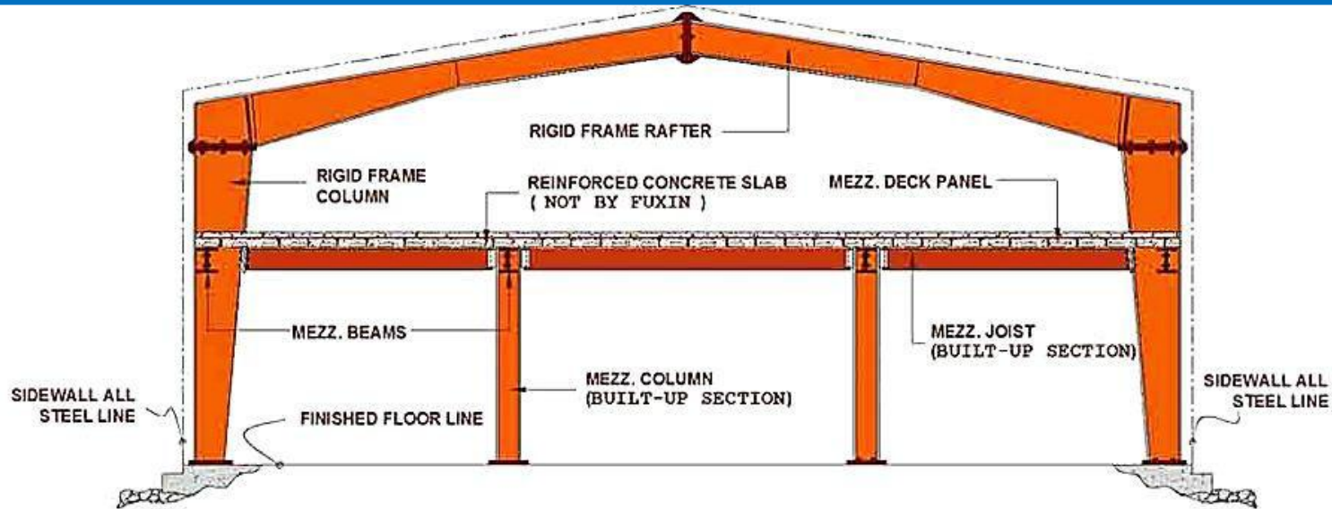
ELEVATION : MEZZANINE CROSS SECTION
