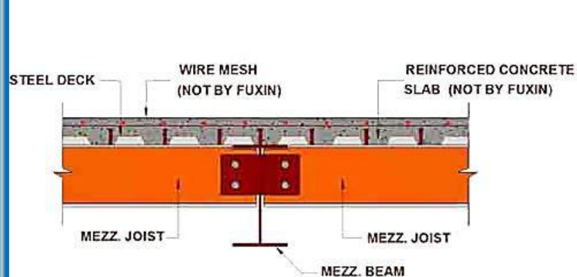
MEZZ. JOIST CONNECTION TO MEZZ. BEAM
